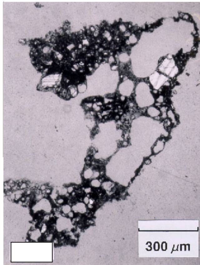
Figure 56 - Thin section photo of a lunar agglutinate. Vesicular glass welds soil particles together. Minute Fe particles are present in the glass.
